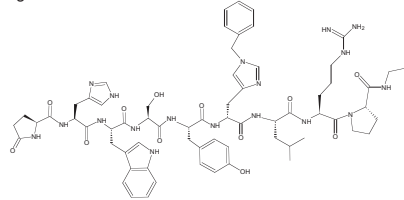
Figure 2. Structure of Histrelin
